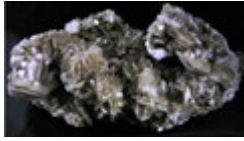
Muscovite, Feldspar, Galileia, Minas Gerais, Brazil.
